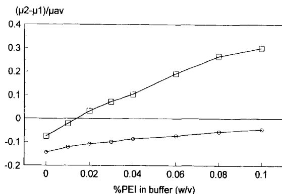
Fig. 6. Relative mobility difference against %PEI in buffer for long peptides using a 5% PEI-coated capillary. The changes in selectivity represented are between peptides WAGGDASGE and ELAGAPPEPA (□), and between SYSMHEPRWG and LQAAPALDKL (○). All the conditions as in Fig. 5.
