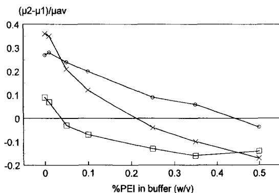
Fig. 4. Relative mobility difference against %PEI in buffer for basic proteins using a 10% PEI-coated capillary. The changes in selectivity represented are between \alpha -chymotrypsinogen and trypsinogen ( \square ), between ribonuclease A and trypsinogen ( \times ) and between ribonuclease A and \alpha -chymotrypsinogen ( \circ ). All the conditions as in Fig. 3.
