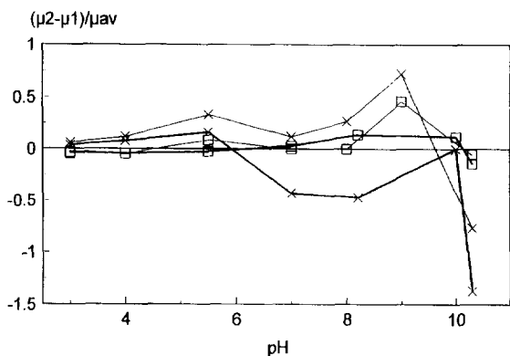
Fig. 3. Relative mobility difference vs. pH for some basic proteins. Narrower lines represent the change in selectivity observed using buffers without PEI. Thicker lines represent the change in selectivity using buffers containing 0.1% PEI. The changes in selectivity represented are between \alpha -chymotrypsinogen and trypsinogen ( \square ) and between ribonuclease A and trypsinogen ( \times ).
