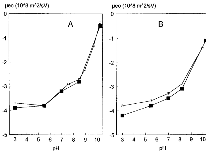
Fig. 1. Plots of electroosmotic flow against pH. Buffers without PEI (A) and with 0.1% PEI as additive (B). Coated capillaries with 5 (■) and 10% (○) PEI were used. Acetone was used as a neutral marker.
